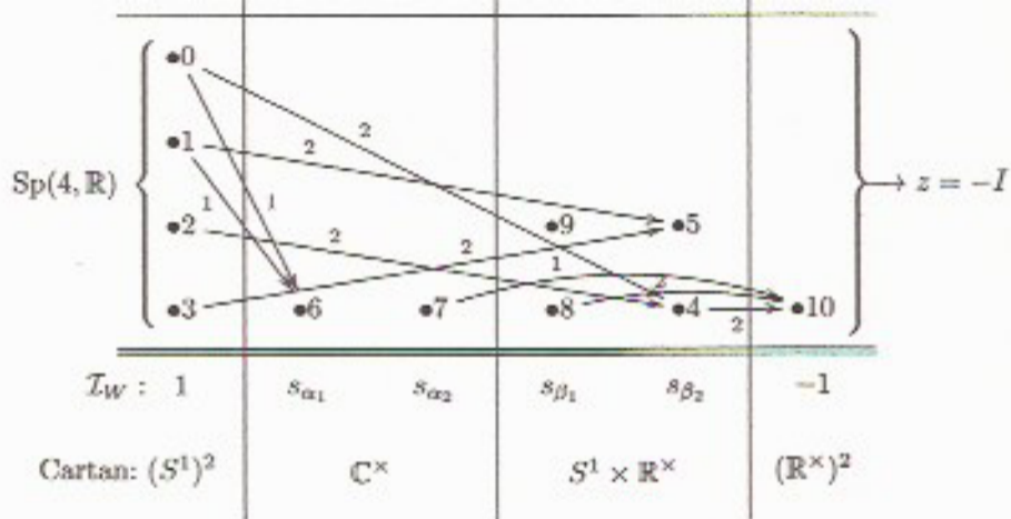
Figure 1: \mathcal{X} and Cayley transforms for Sp(4)
